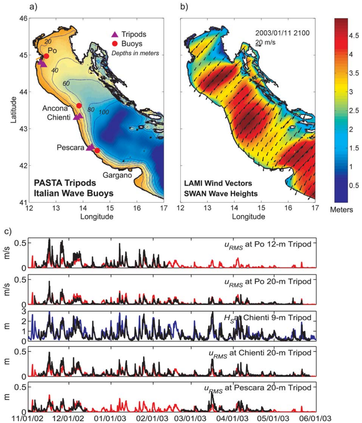
Figure 4. (a) Wave data were recorded by pressure and velocity sensors on the EuroSTRATAFORM tripods, and by a network of wave-monitoring buoys maintained by the Italian Agency for Environmental Protection. (b) The SWAN model was forced with LAMI wind fields (black arrows) and produced fields of wave heights. The colors shown here are results for a January Bora event with red = 5 m significant height. (c) The model results (black) usually compare favorably with measured wave heights (blue) and near-bottom orbital velocities (red).
